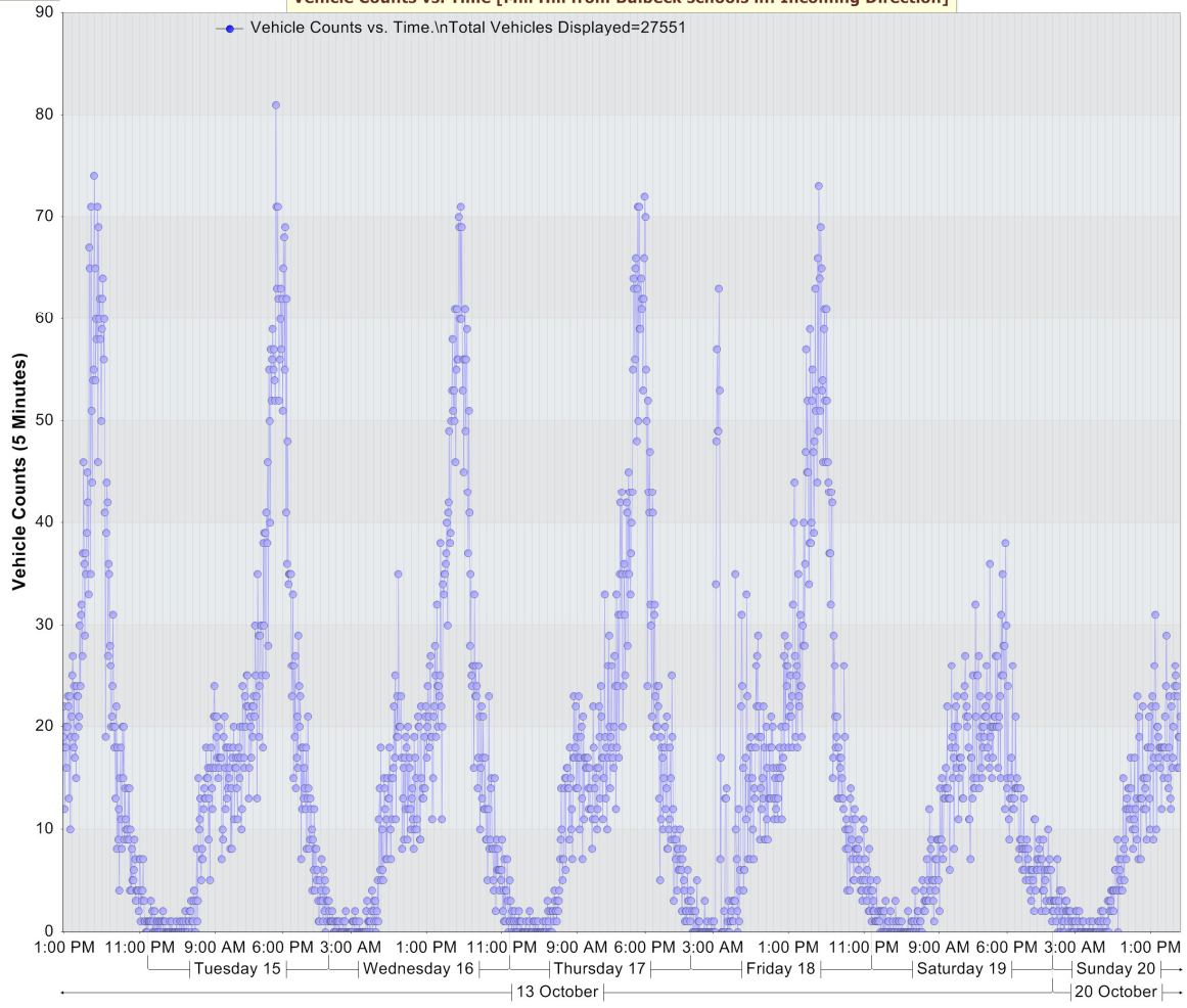
Vehicle Counts vs. Time [Mill Hill from Bulbeck schools in: Incoming Direction]
